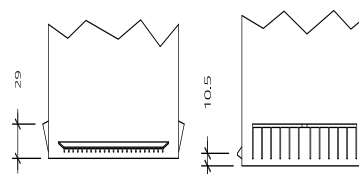
Base plate B07
